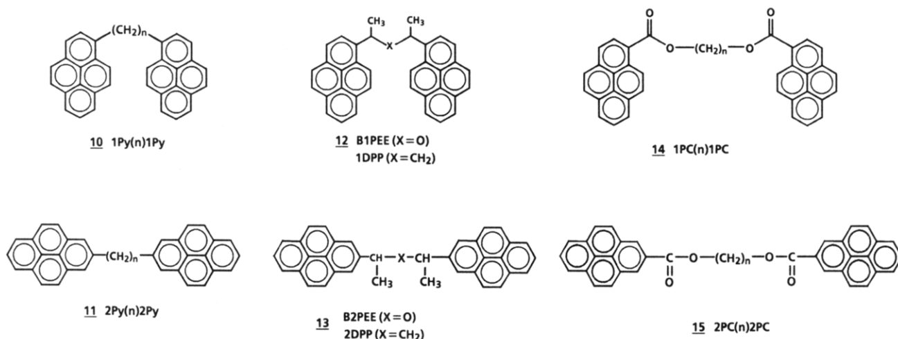
Figure 15. Chemical structures of bis-pyrenyl compounds.
