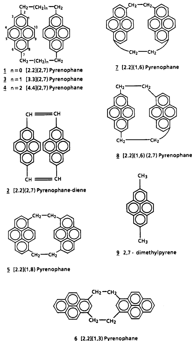
Figure 13. Chemical structures of pyrenophanes.
