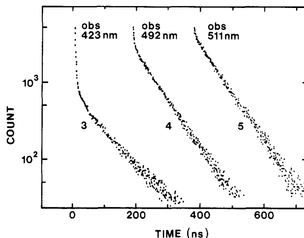
Figure 8. Fluorescence decay curves of the excimer monitored at different wavelengths in a solution of HPC-Py/56 in water, 20 °C. Reprinted from 21. Copyright 1987 American Chemical Society.
