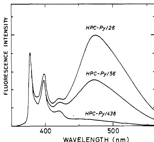
Figure 7. Fluorescence spectra of HPC-Py (0.026 g L -1 ) in water; \lambda_{exc} = 330 nm; 20 °C; spectra were normalized at 377 nm. Reprinted from ref 144. Copyright 1992 American Chemical Society.
