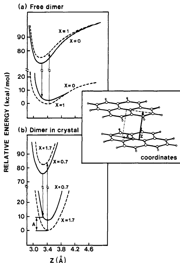
Figure 2. Calculated ground state and excimer potential surfaces for the free pyrene dimer (a) and for the dimer in the pyrene crystal (b). Reprinted from 14. Copyright 1974 Elsevier.
