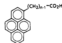
16 n = 4 to 15
